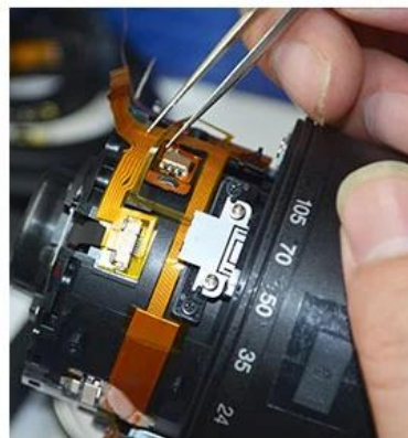
Maintenance disassembly
